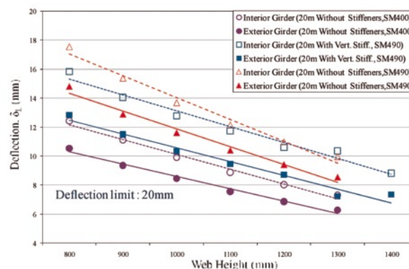
Figure 6 Deflections due to Live Load, L=20m
