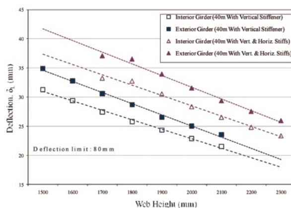
Figure 15 Deflections due to Live Load, L=40m
