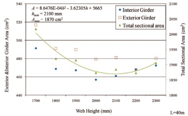
Figure 13 Optimum Girder Height for L=40m (with vert. & horiz. Stiffs., SM490Y)
